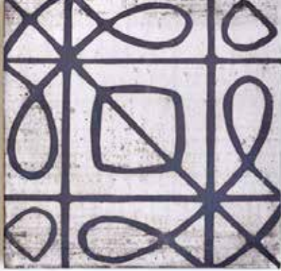
6" Pattern #9: Cast Iron (Chladni Figure 54)
