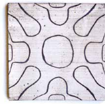
6" Pattern #5: Cast Iron (4957 Hz)
